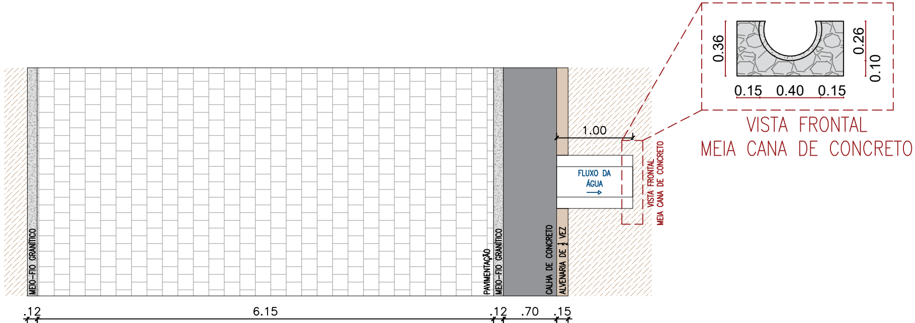
Vista superior – ST03 escala → 50
